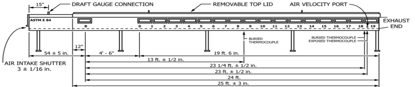
Diagram 1. Test Chamber side view showing critical dimensions.
